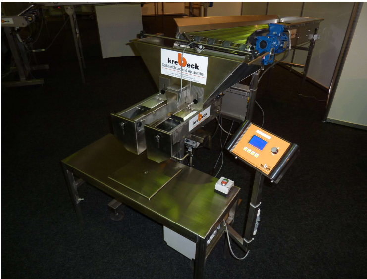
Dosing System ADS 80/2 Crate Feeder with weighing unit
